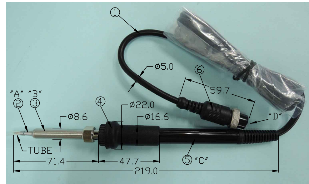
VIEW C
